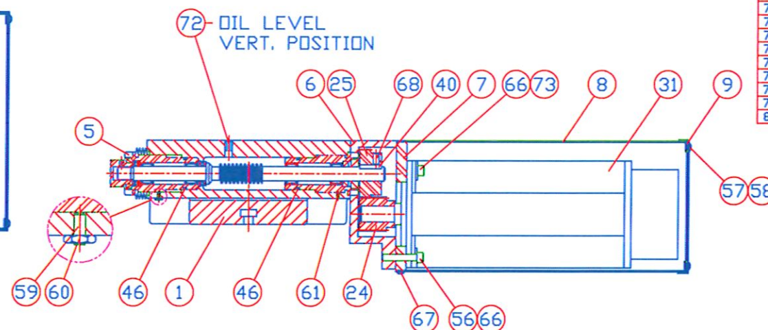
SECTION C-C
